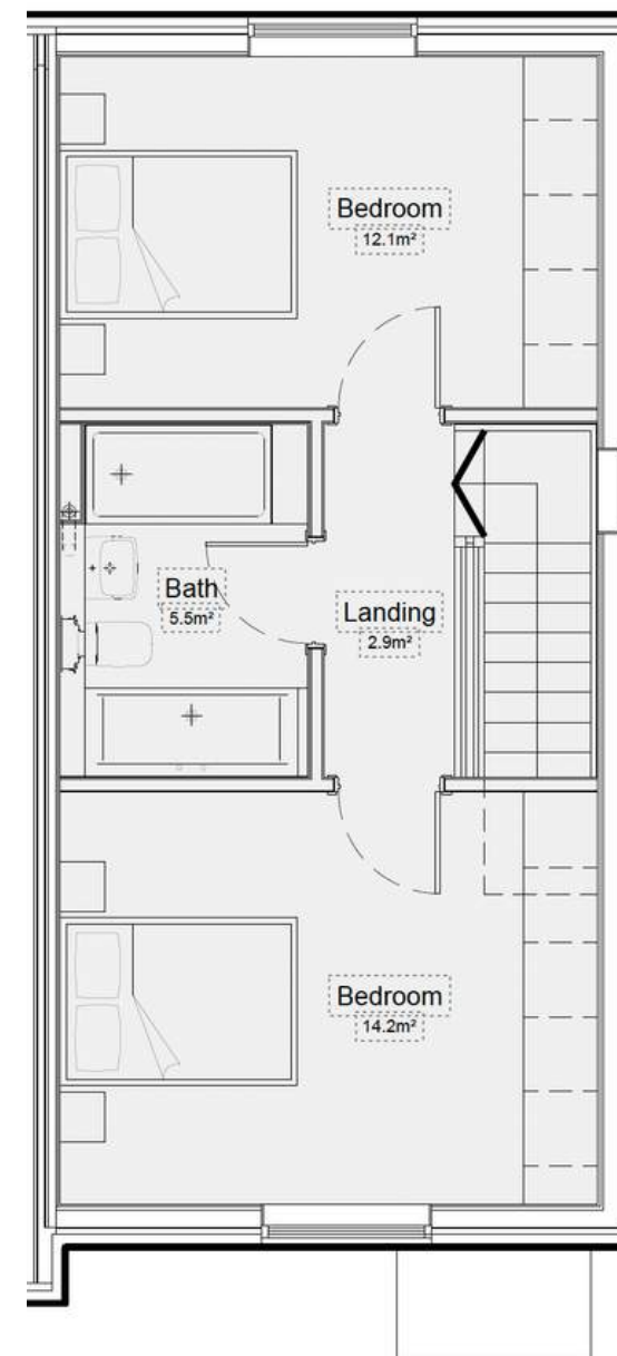
Second floor
