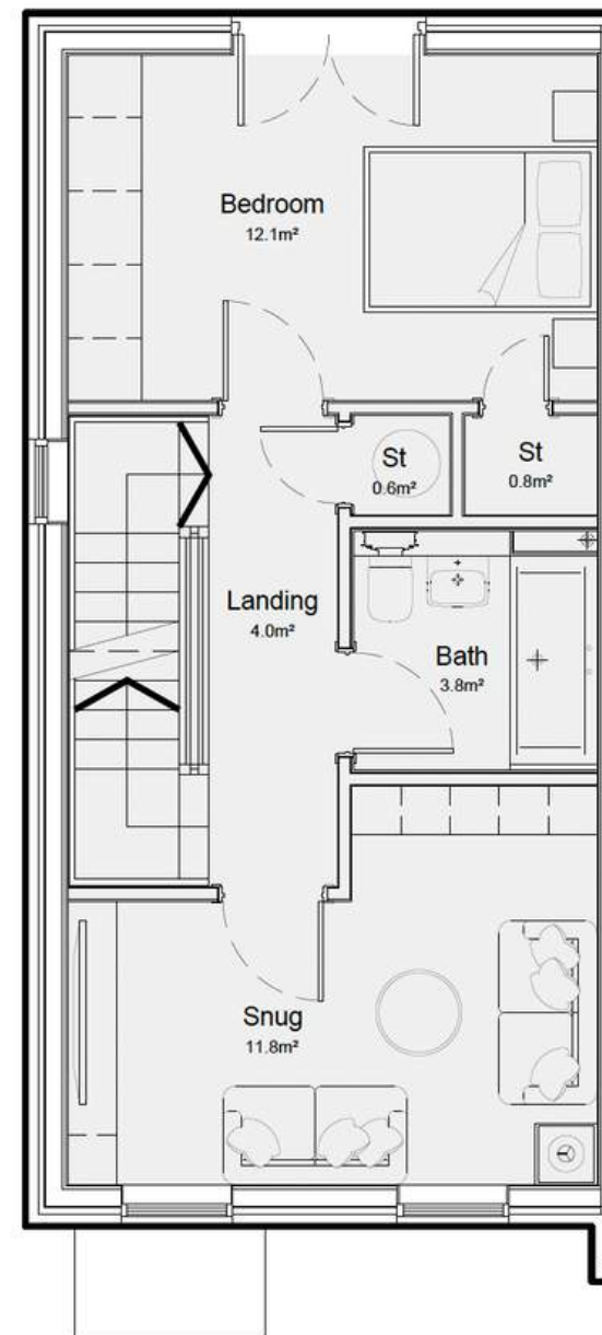
First floor
