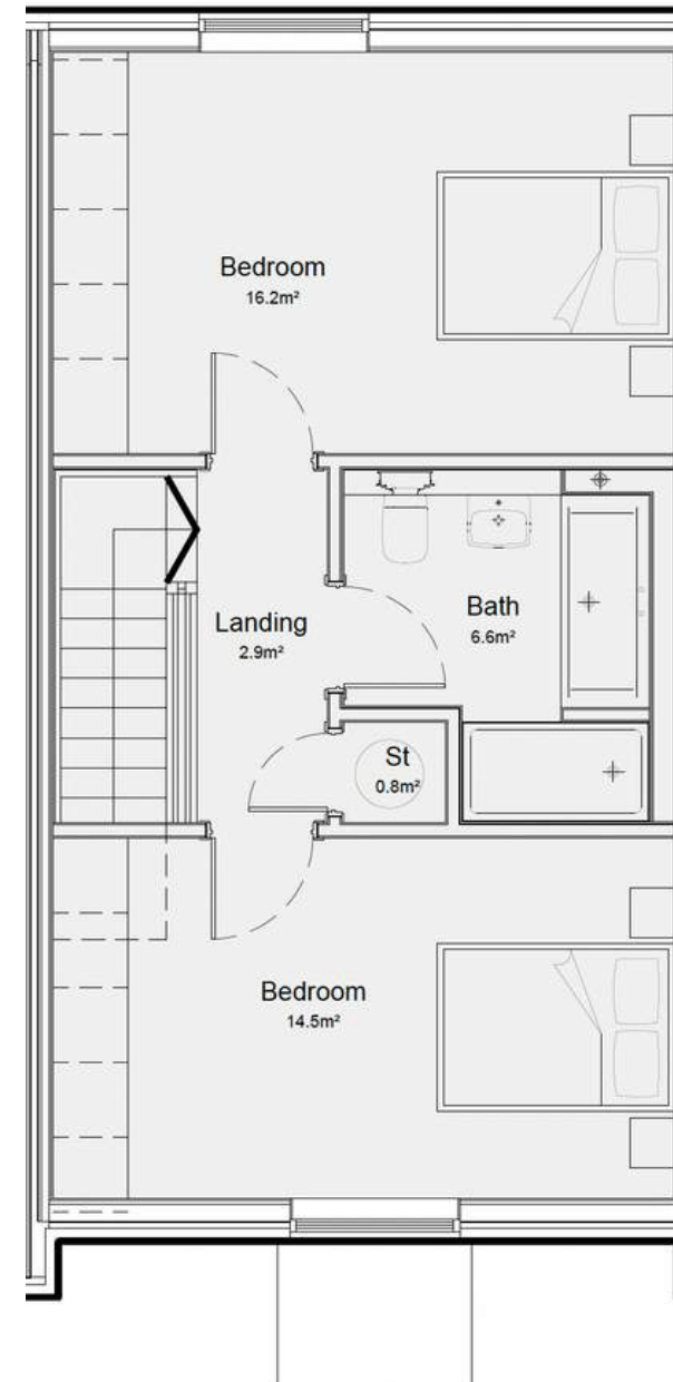
Second floor
