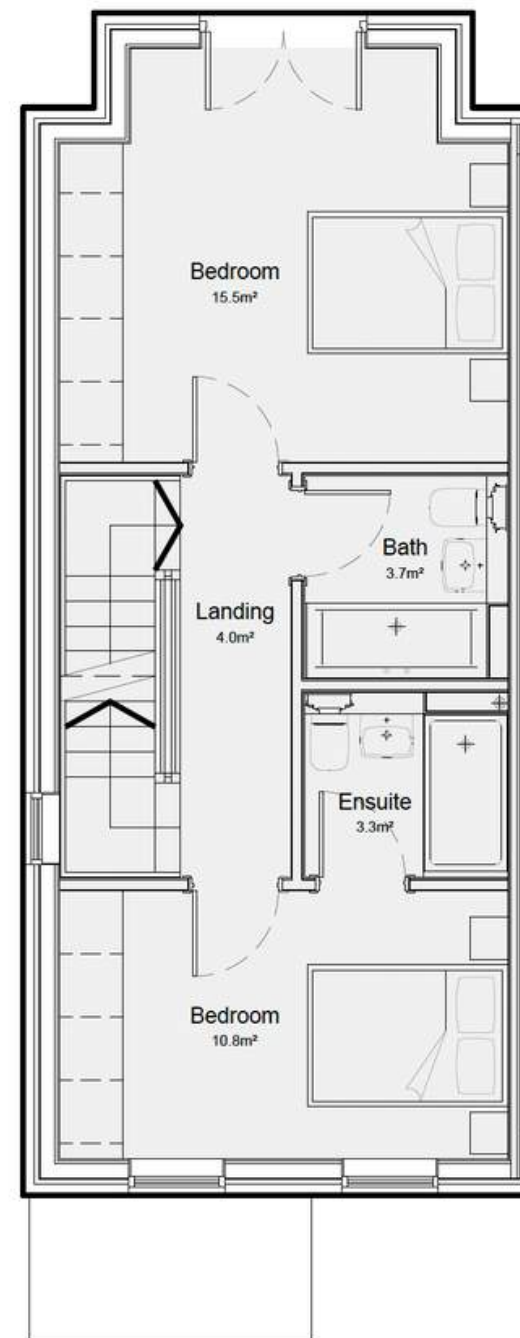
First floor
