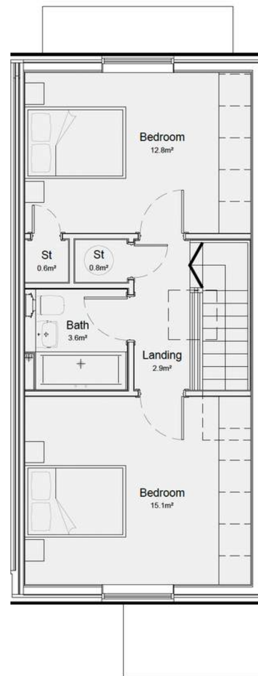
Second floor
