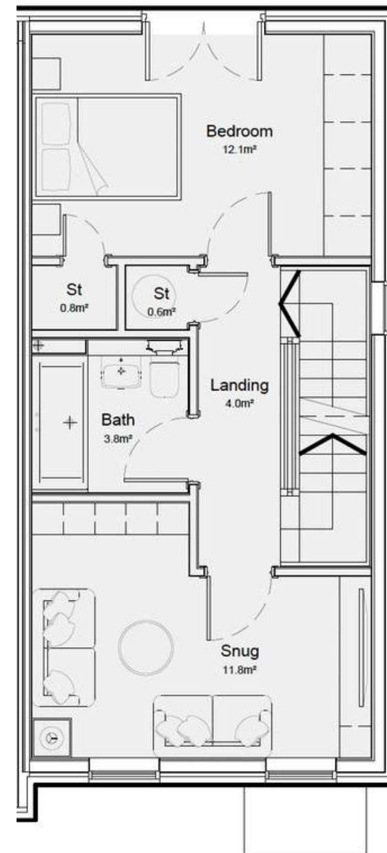
First floor
