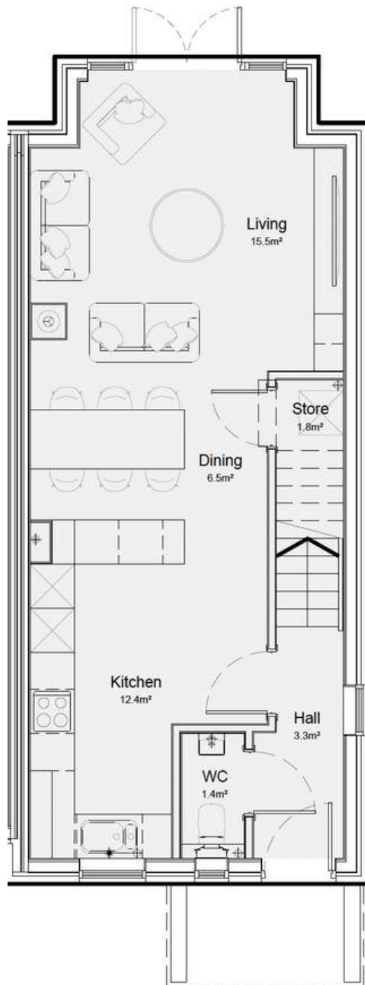
Ground floor
