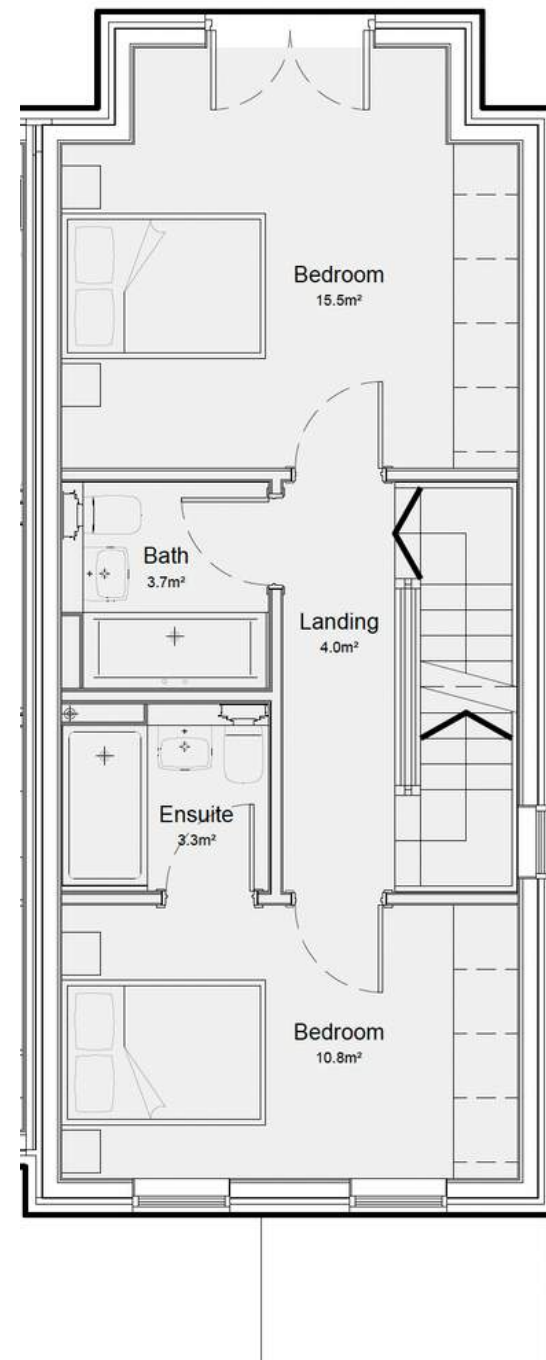
First floor
